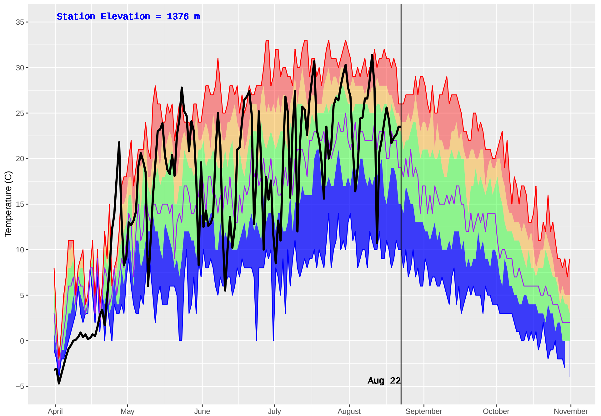
DUNCAN (385) : Historical (1981–2016) and Current (2018) Daily Temperature
