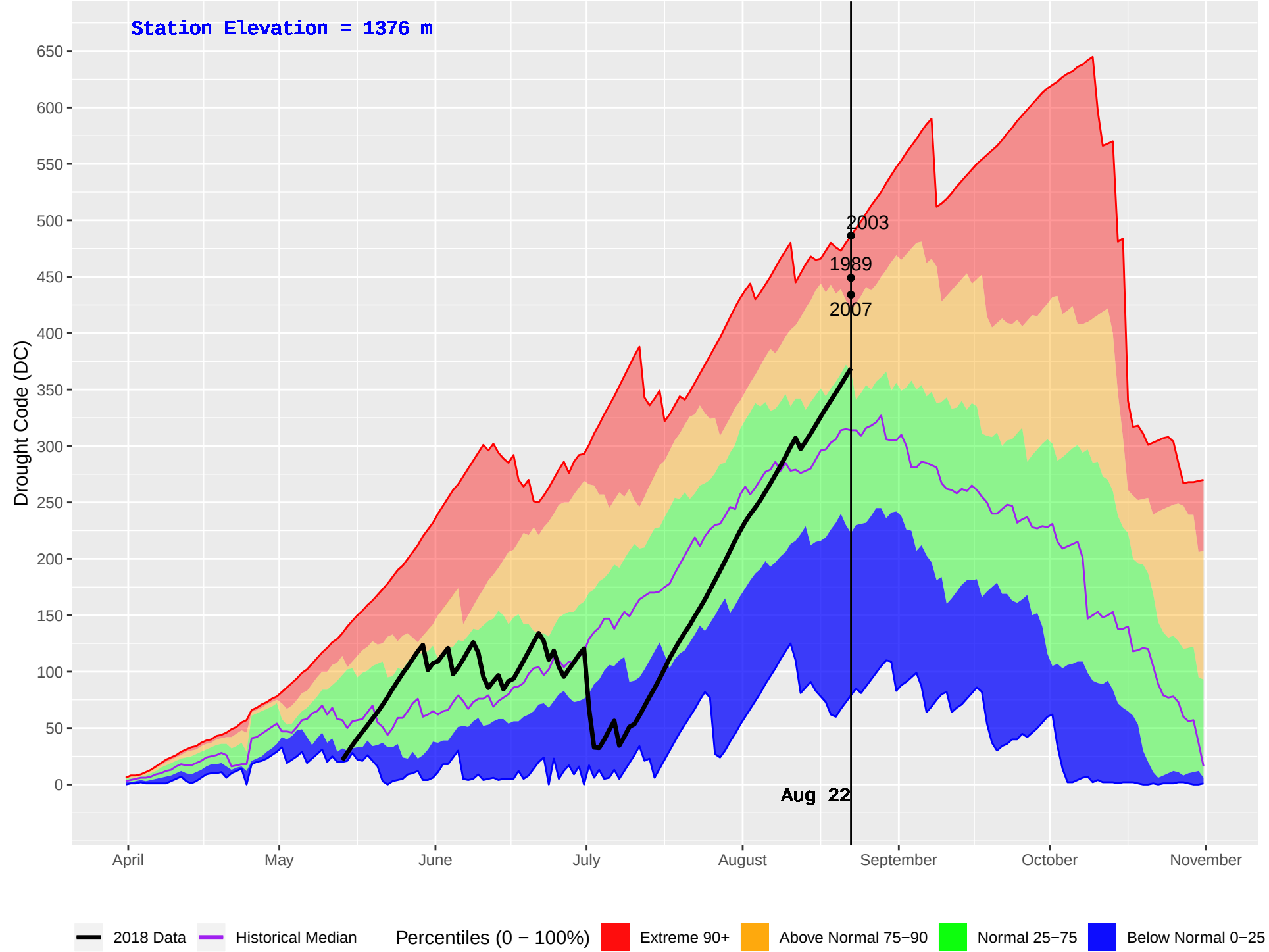
DUNCAN (385) : Historical (1981–2016) and Current (2018) Daily Drought Code (DC)
