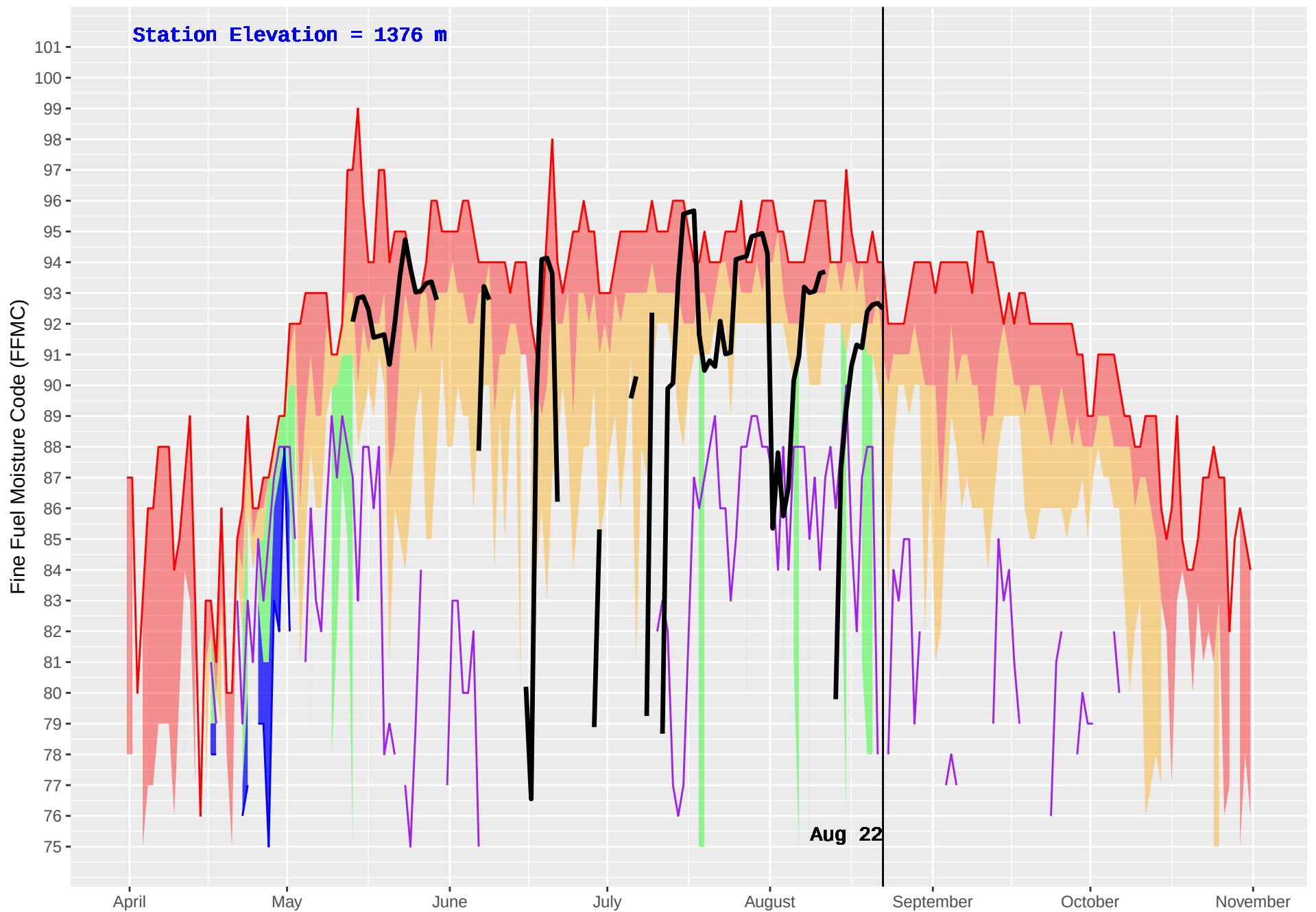
DUNCAN (385) : Historical (1981–2016) and Current (2018) Daily Fine Fuel Moisture Code (FFMC)
