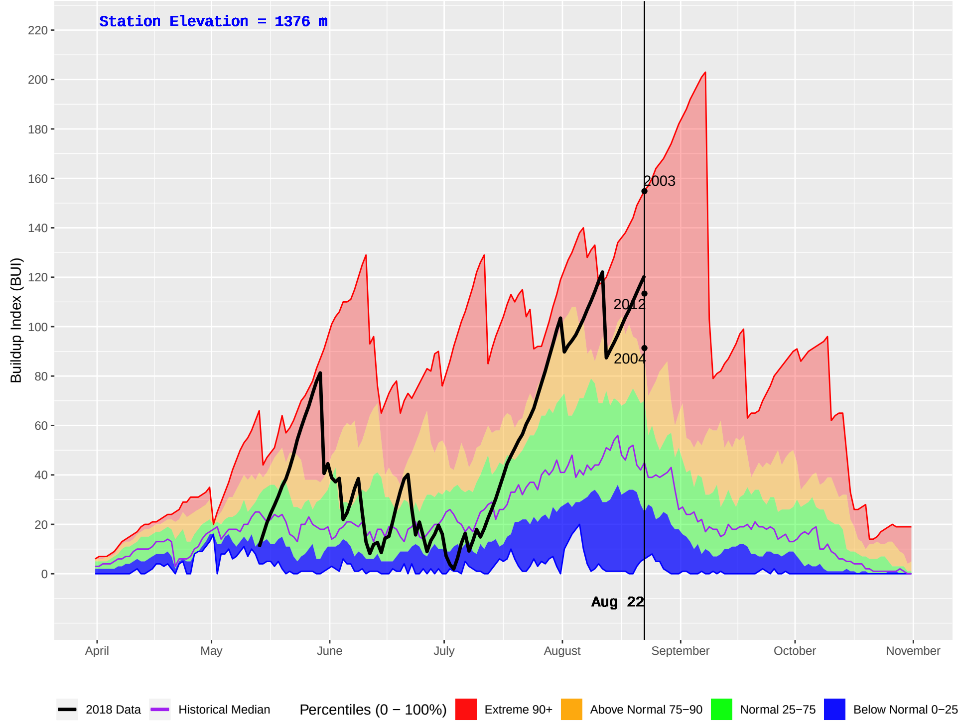
DUNCAN (385) : Historical (1981–2016) and Current (2018) Daily Buildup Index (BUI)
