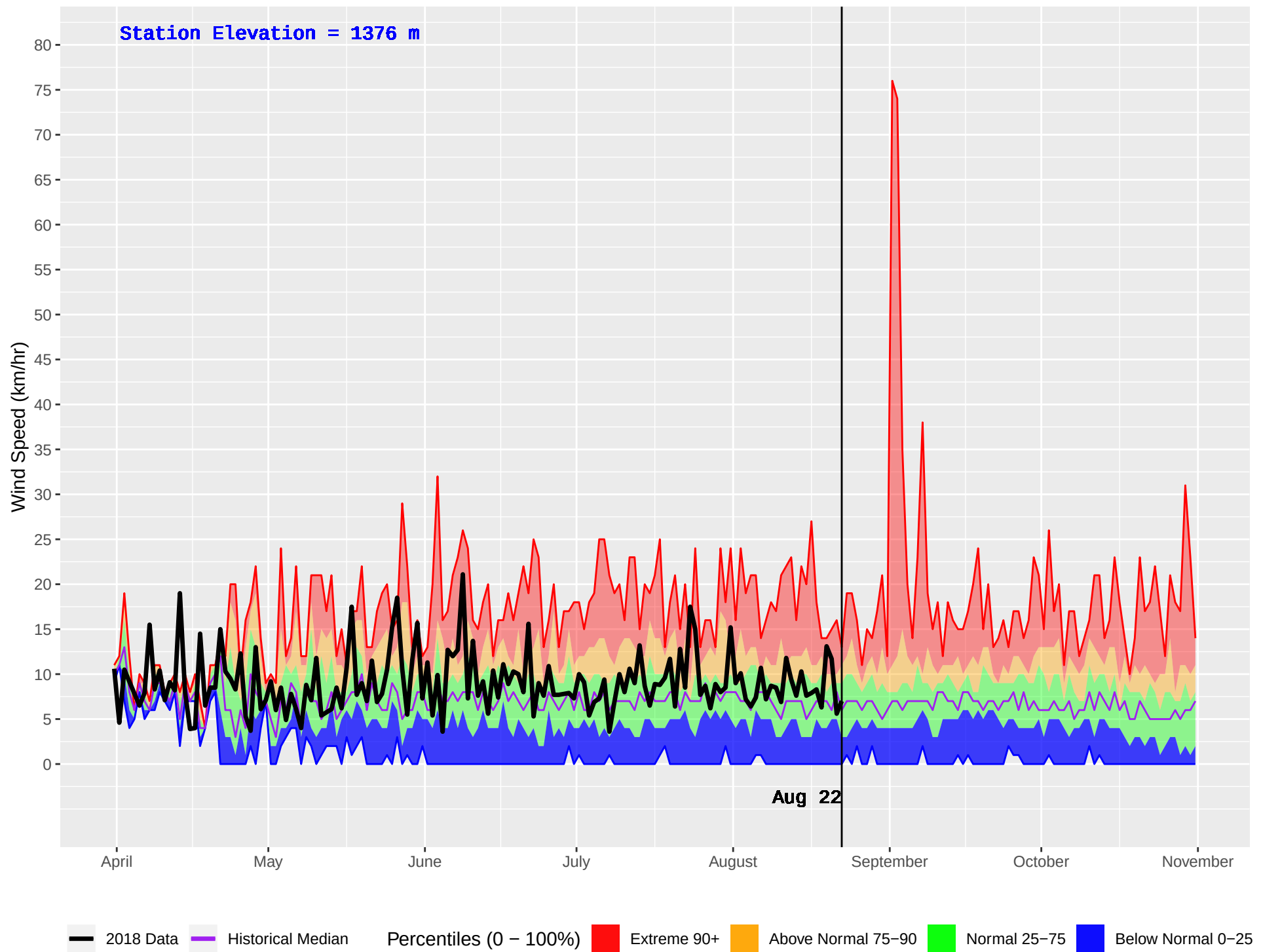
DUNCAN (385) : Historical (1981–2016) and Current (2018) Daily Wind Speed
