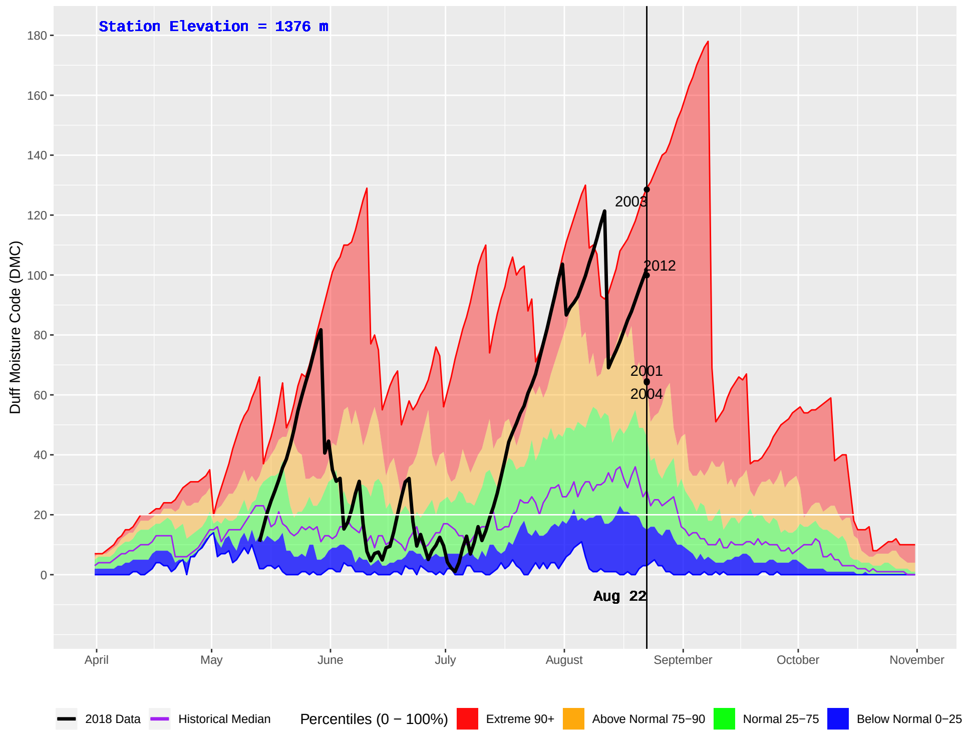
DUNCAN (385) : Historical (1981–2016) and Current (2018) Daily Duff Moisture Code (DMC)
