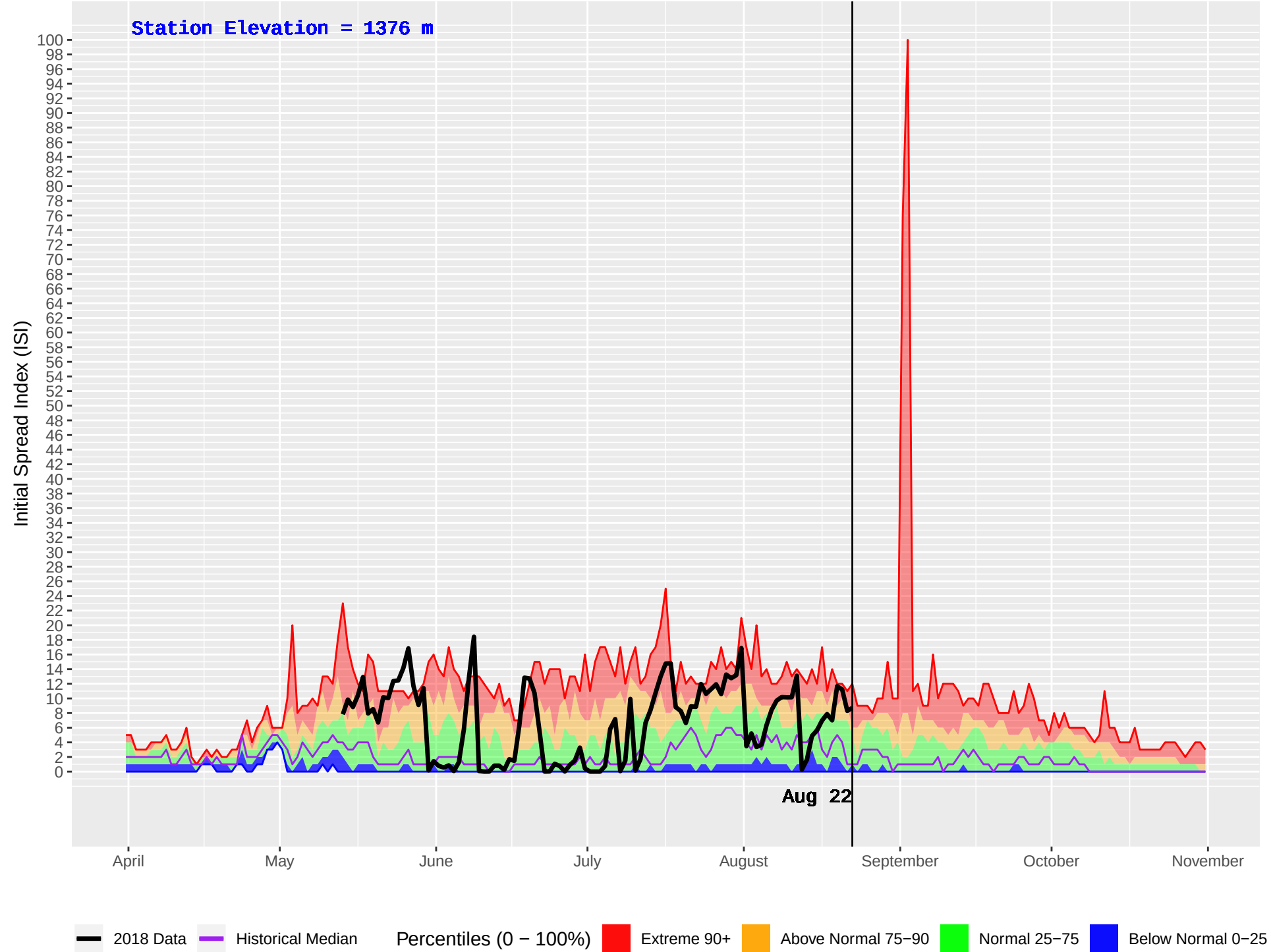
DUNCAN (385) : Historical (1981–2016) and Current (2018) Daily Initial Spread Index (ISI)
