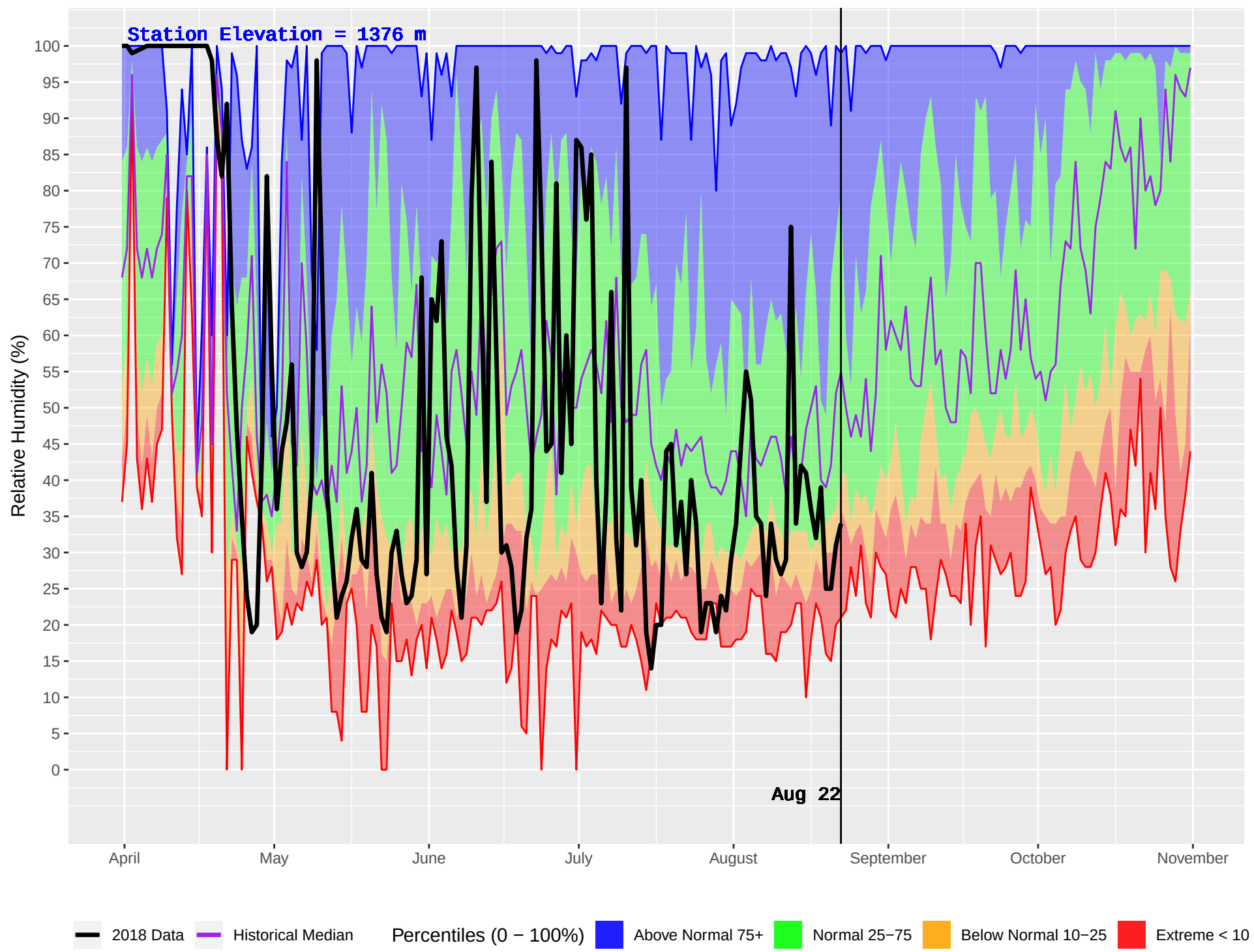
DUNCAN (385) : Historical (1981–2016) and Current (2018) Daily Relative Humidity
