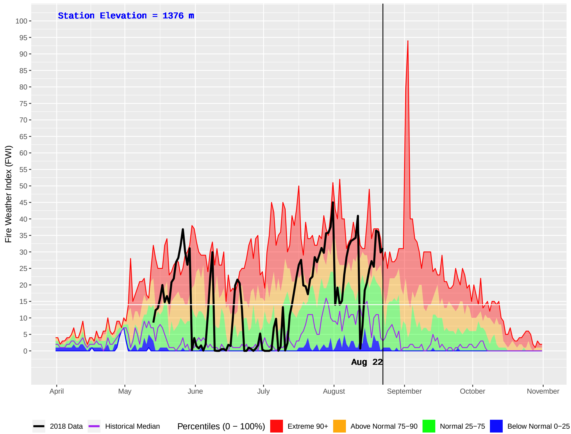
DUNCAN (385) : Historical (1981–2016) and Current (2018) Daily Fire Weather Index (FWI)
